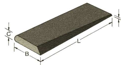
Multiformstein
